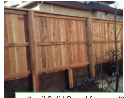
● 3-rail Solid Board fence w/2x6 cap on Retaining Wall using concealed Steel Posts
